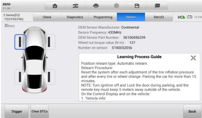
Figure 5-27 Relearn Function Main Screen
