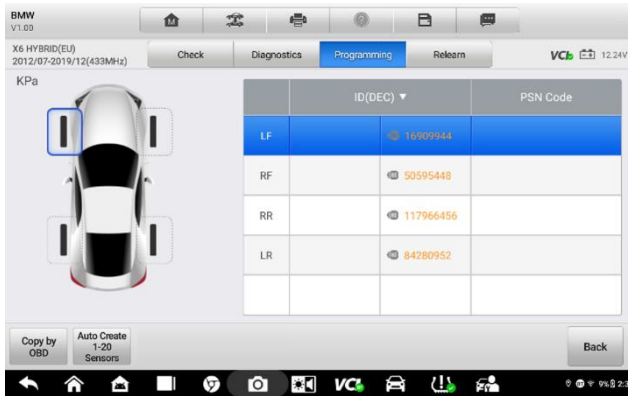
Figure 5-25 Copy by OBD Function Main Screen
