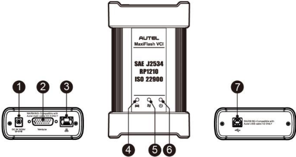
Figure 2-4 MaxiFlash VCI
