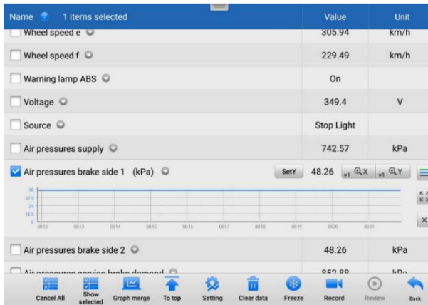
Figure 4-14 Waveform Graph Mode Screen
