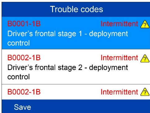
Figure 3-9 Sample SRS Trouble Codes Screen
