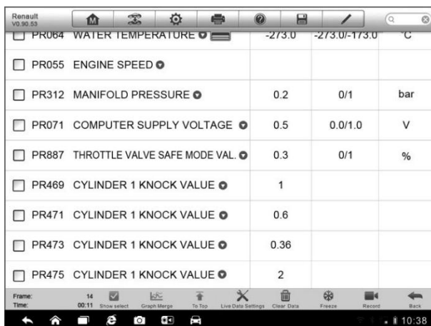
Figure 4-10 Sample Live Data Screen
