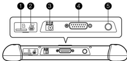
Figure 2-3 MaxiSys MS906 Tablet Top View
