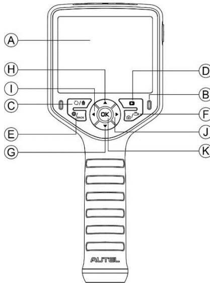
Figure 2-5 MaxiVideo MV460 Buttons and Controls
