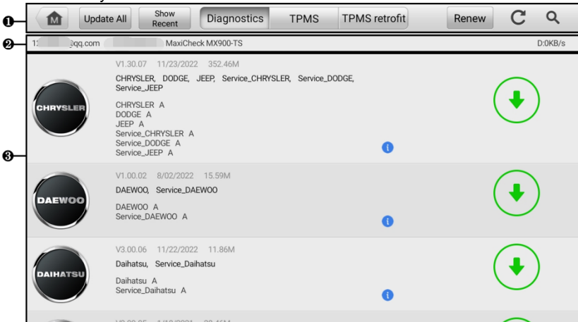
Figure 11-1 Update Screen
