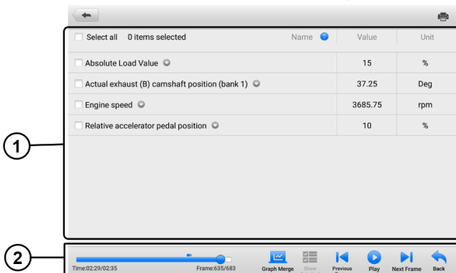
Figure 7-6 Data Playback Screen
