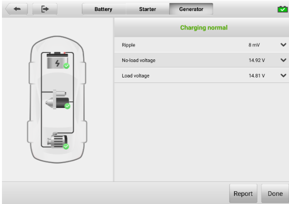
Figure 8-8 Generator Test Results Screen
