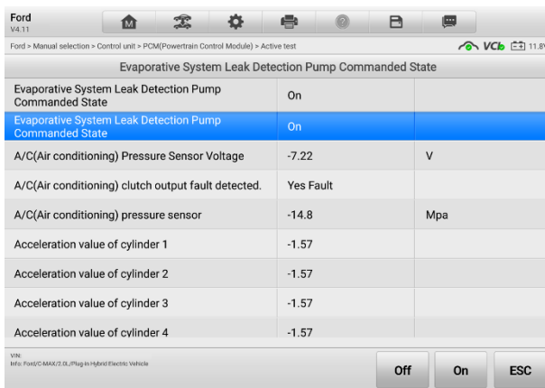
Figure 4-17 Active Test Screen
