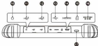
Figure 2-3 MaxiSys Tablet, Top View
