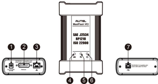
Figure 2-4 MaxiFlash VCI
