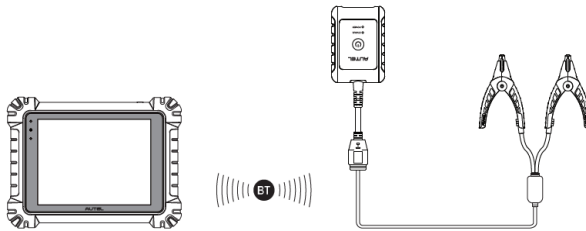
Figure 8-2 Connecting with the Tablet
