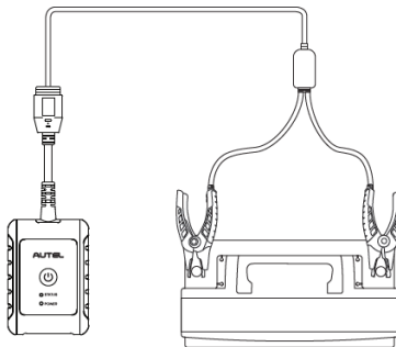
Figure 8-3 Connecting to a Battery
