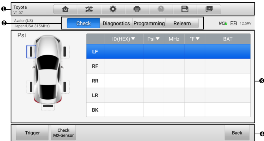
Figure 6-8 TPMS Service Screen
