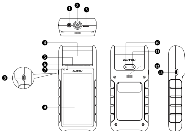
Figure 2-1 MaxiBAS BT608E Front/Back/Side View
