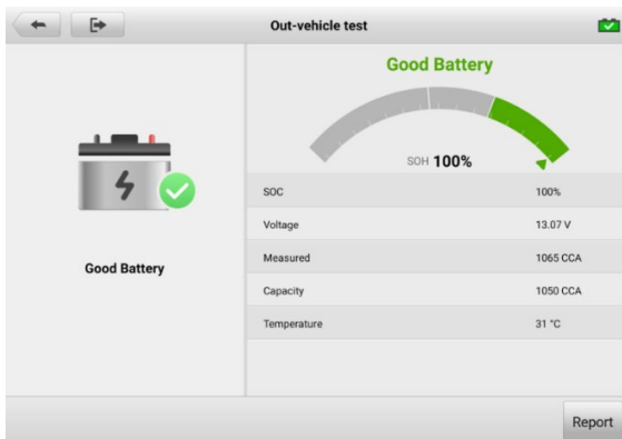
Figure 10-10 Out-vehicle Test Results Screen
