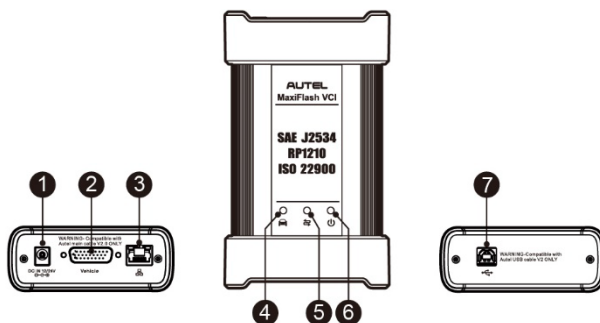
Figure 2-5 MaxiFlash VCI Programming Device
